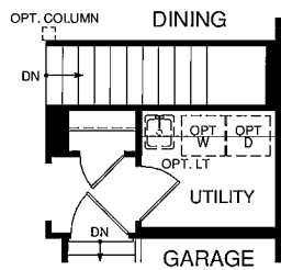
PARTIAL FIRST FLOOR PLAN w/ OPT. BASEMENT PLAN
