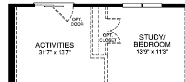
PARTIAL BASEMENT PLAN w/ OPT MORNING ROOM @ WALKOUT CONDITION
