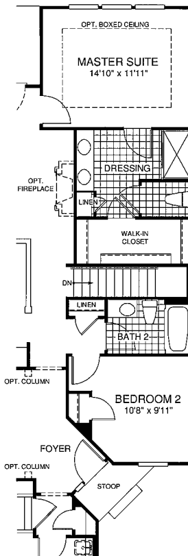
PARTIAL FIRST FLOOR PLAN w/ OPT. BASEMENT COND.
