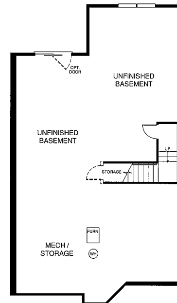
OPT. BASEMENT PLAN
