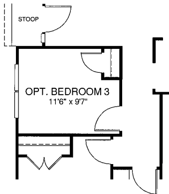
PARTIAL FIRST FLOOR PLAN w/ OPT. BEDROOM 3
