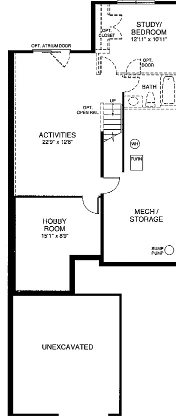
OPT. FINISHED BASEMENT PLAN
